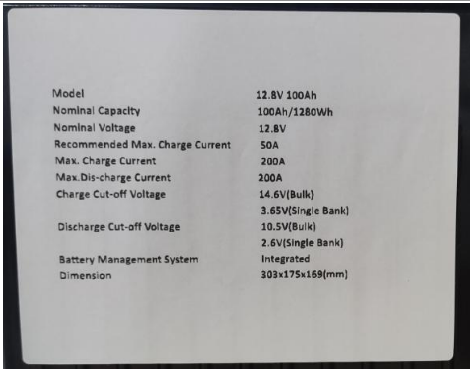
Photo 3 标签特写 Label close-up
